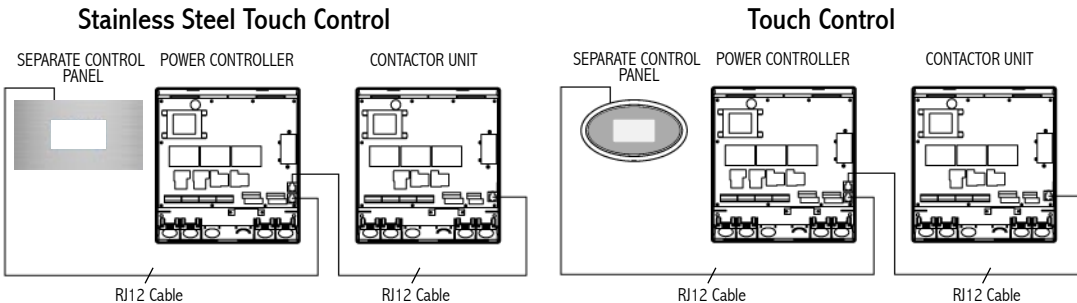
Fig.5 Installation of separate Control Panel and Power Controller with Contactor Unit
